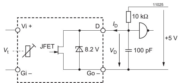
Fig. 15 Test circuit with definition of voltage V_D and current I_D
