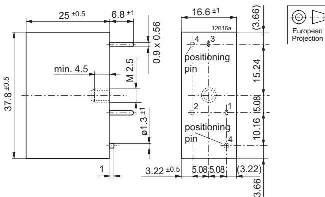
Fig. 22 Mechanical data of FP filters. Weight approx. 30 g
