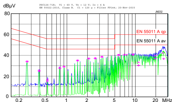
Fig. 11a PSC126-7iR: Conducted disturbances at the input as per EN 55011, at V_i = 60 V, V_o = 12 V, I_o = 6 A. External C_i = 120 μF + Filter FP144.
