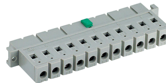
Fig. 23 Different mating connectors, including code key system
