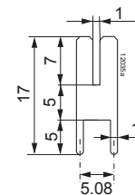
Fig. 19 Solder tag HZZ01204-G. Delivery content: 10 pieces
